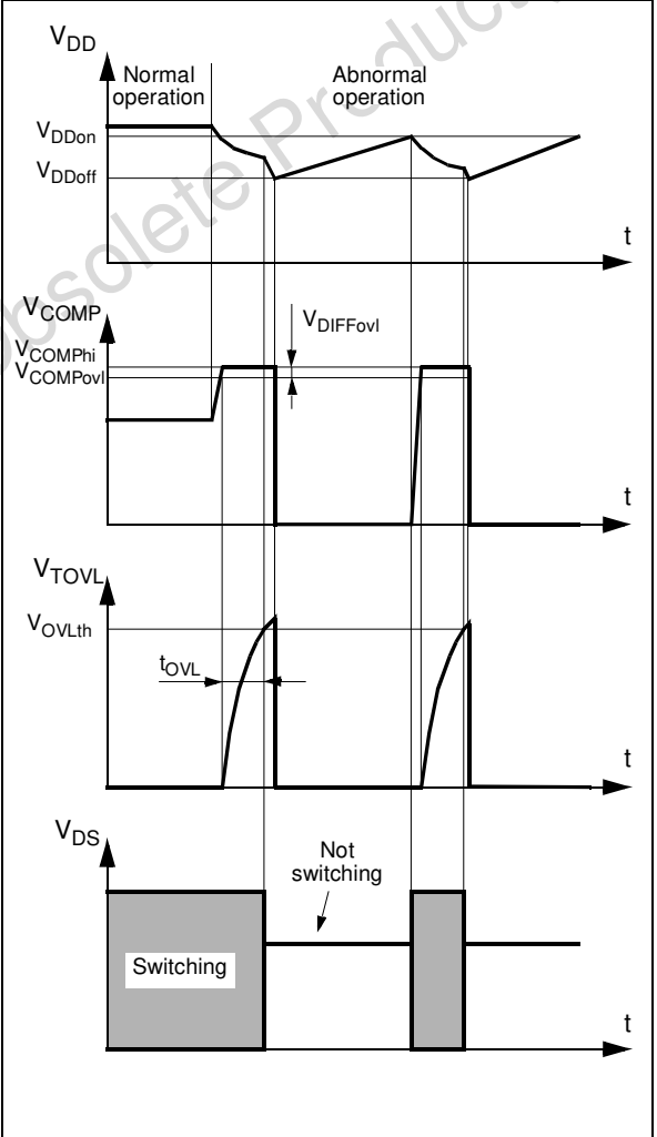
Figure 4: Overload event
